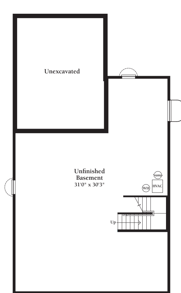
Standard Lower Level Floor Plan Elevation A
