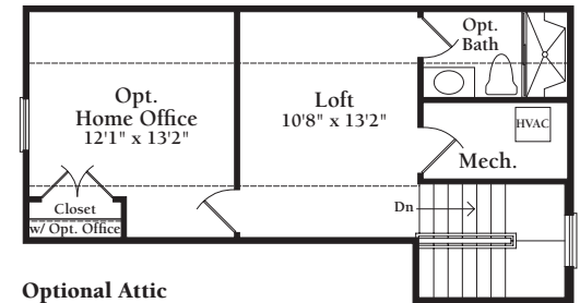
Optional Attic w/ Opt. Home Office and Opt. Bath
