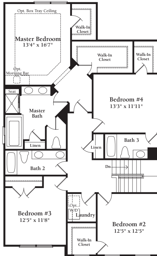
Partial Upper Level Floor Plan Alternate Master Bath
