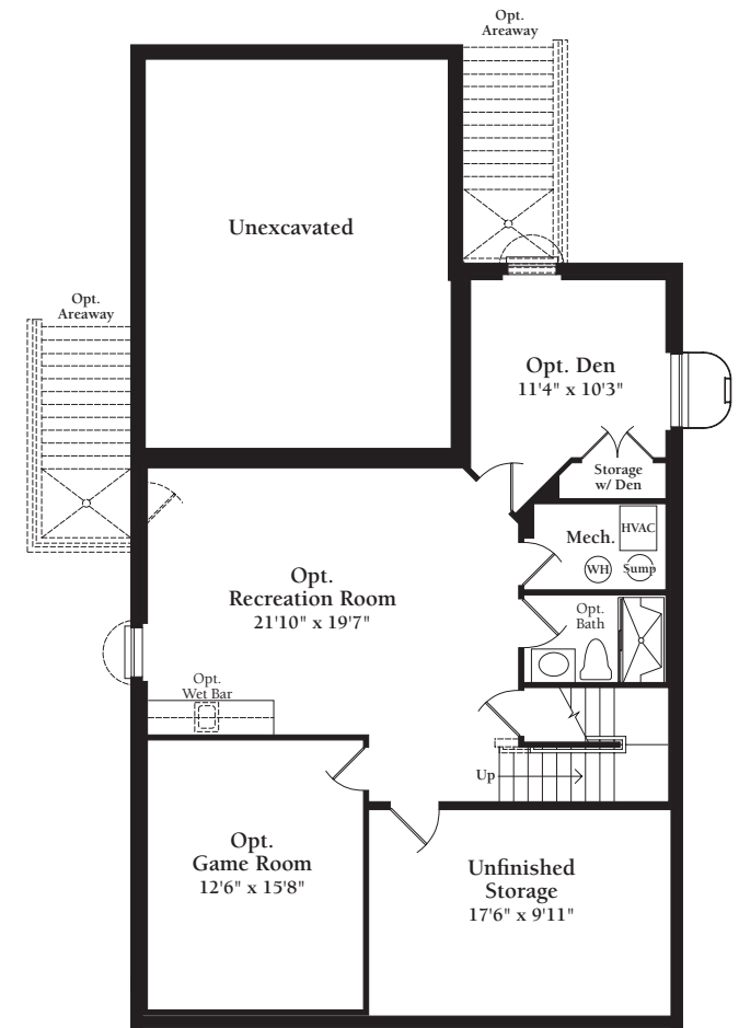
Optional Lower Level Floor Plan w/ Opt. Finished Spaces, Opt. Wet Bar, Opt. Areaway, and Opt. Bath Elevation A
