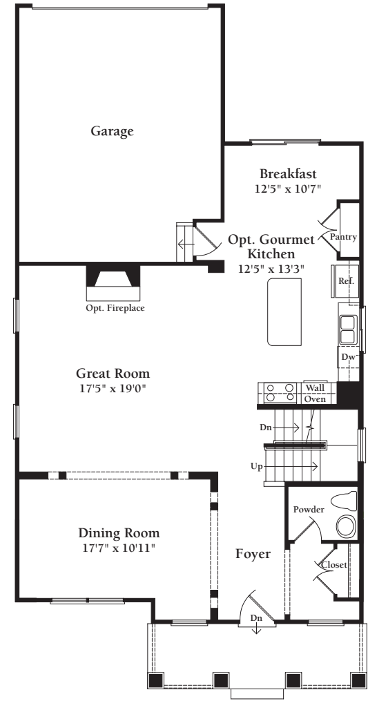
Optional Main Level Floor Plan w/ Stairs to Opt. Finished Basement, Opt. Gourmet Kitchen and Opt. Fireplace Elevation C
